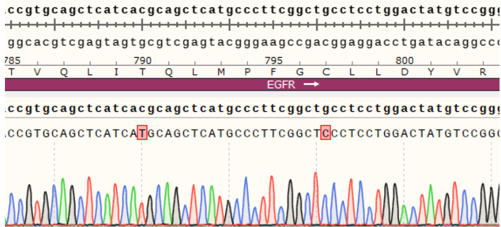
Figure 3 | The EGFR mutation analysis by Sanger sequencing.
