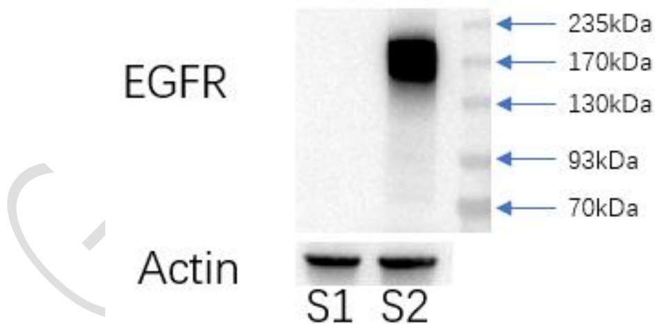
Figure 2 | The protein expression levels of Human EGFR(T790M-C797S) in the H_EGFR(T790M-C797S) BAF3 Cell Line(Cat. GM-C29679) were determined by Western blotting (WB).
