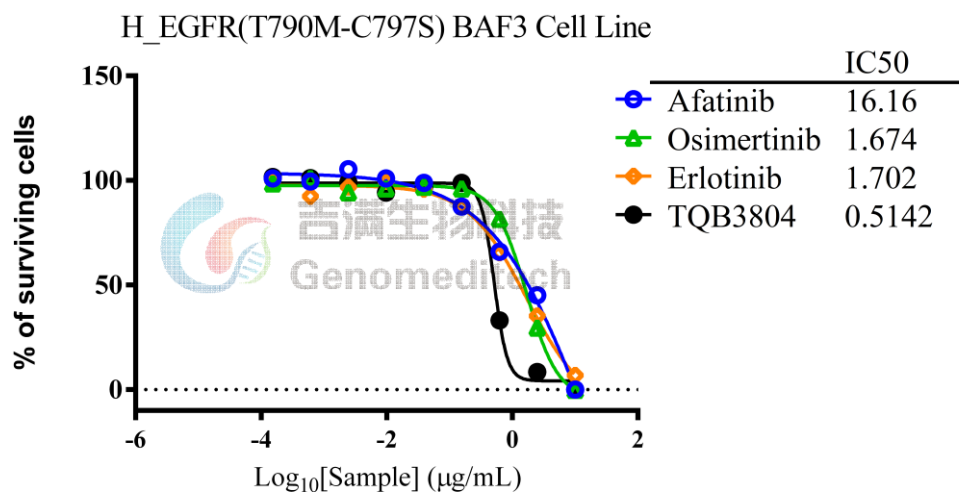
Figure 1 | Cell proliferation assay. The H_EGFR(T790M-C797S) BAF3 Cell Line (Cat. GM-C29679) at a concentration of 1E4 cells/well (96-well format) was treated with serial dilutions of Osimertinib (AZD9291) (Selleck/S7297), Erlotinib (OSI-774) (Selleck/S7786), Afatinib (BIBW2992) (Selleck/S1011), EGFR-IN-7(TQB3804)(BioChem Partner/BCP34208) in assay buffer (RPMI 1640 + 10% FBS + 1% P.S) for 72 hours. The firefly luciferase activity was measured using the GMTiter™ Luminescent Cell Viability Assay (Cat. GM-040504).
